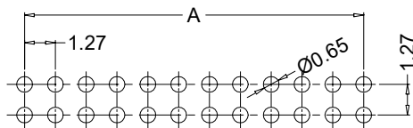
Recommended P.C.B Layout General Tolerance±0.05
