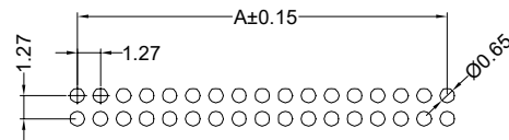
P.C.B Board Layout
